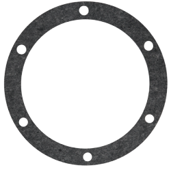
Gasket - 5.5" Bolt Circle Part No HC-3009 Stk. Code 54264
